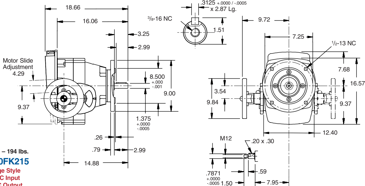
Handwheel Shaft Dimensions
