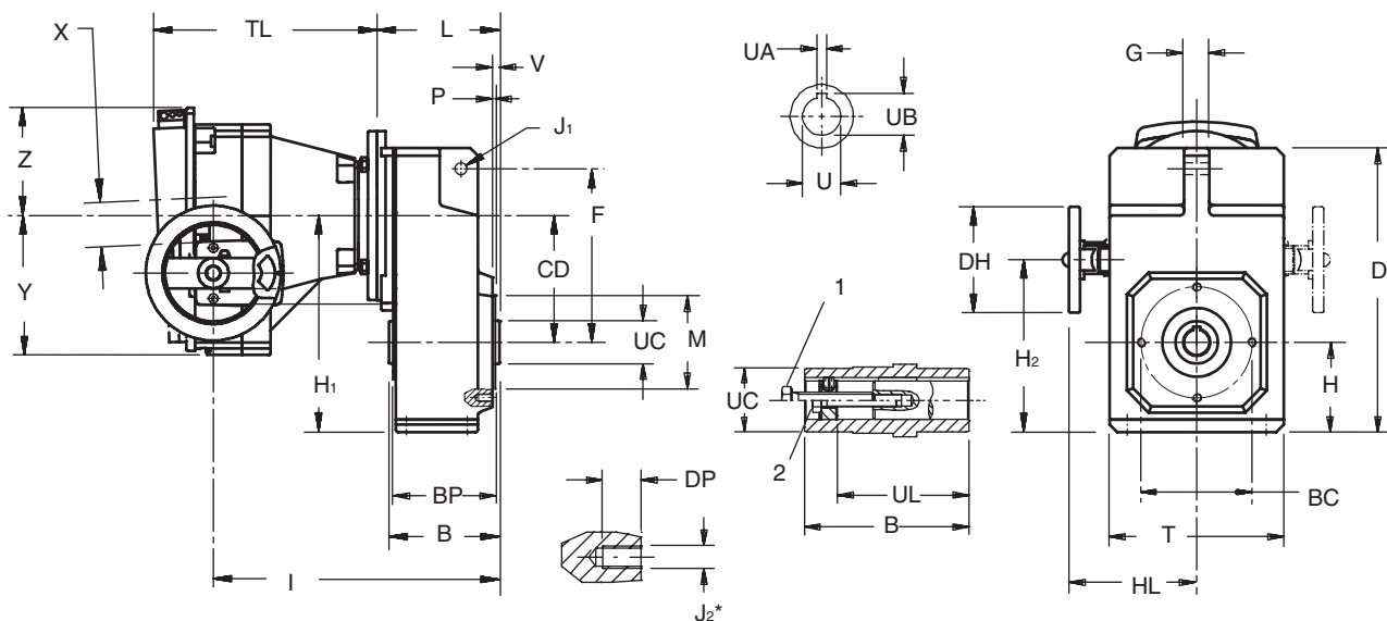
Drawing for Units F102AG — F603AG
